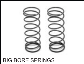
67453 Gray/76mm/52gf (2pcs) 67454 White/76mm/59gf (2pcs) 67455 Blue/76mm/63gf (2pcs) 67456 Orange/76mm/74gf (2pcs) 67457 Green/96mm/40gf (2pcs) 67458 Yellow/96mm/44gf (2pcs) 67459 Red/96mm/49gf (2pcs)
