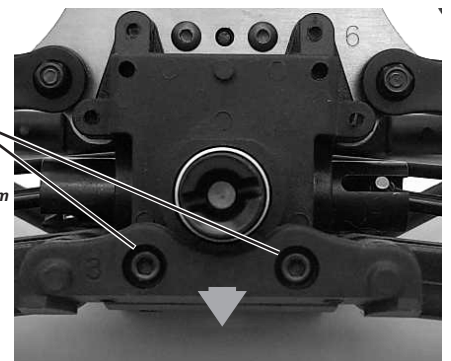
94675 Cap Head Screw M3.5x14mm Inbusschraube M3.5x14mm Vis tête cylindrique M3.5x14mm キャップネジ M3.5x14mm
